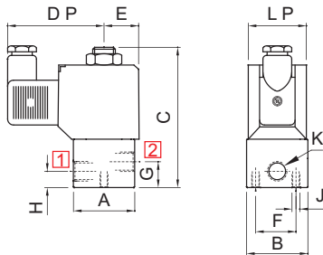
PLUG IN SOLENOID TYPE 22
