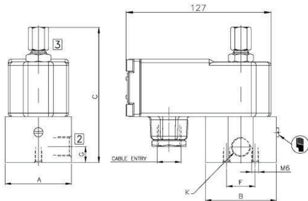
BCE SOLENOID/ Ex d TYPE 87
