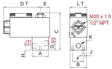
TERMINAL BOX/ Ex d TYPE 16, 19, 37, 39, 58, 58LT
