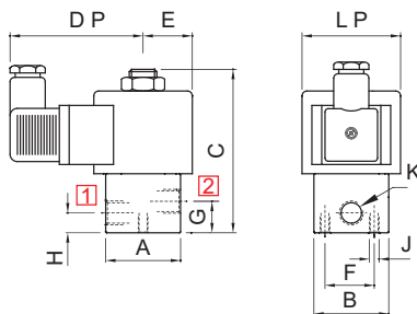
PLUG IN SOLENOID TYPE 25
